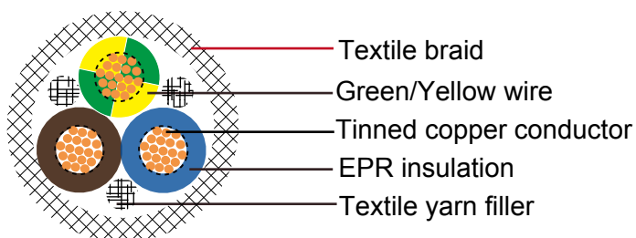
H03RT-H
